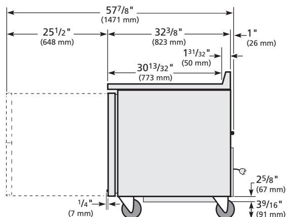
RIGHT VIEW
