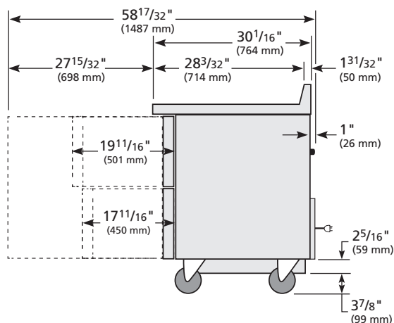
RIGHT VIEW
