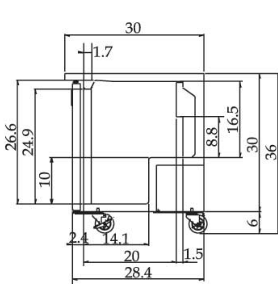
SIDE VIEW
