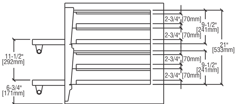
RH SIDE VIEW P44S-BL
