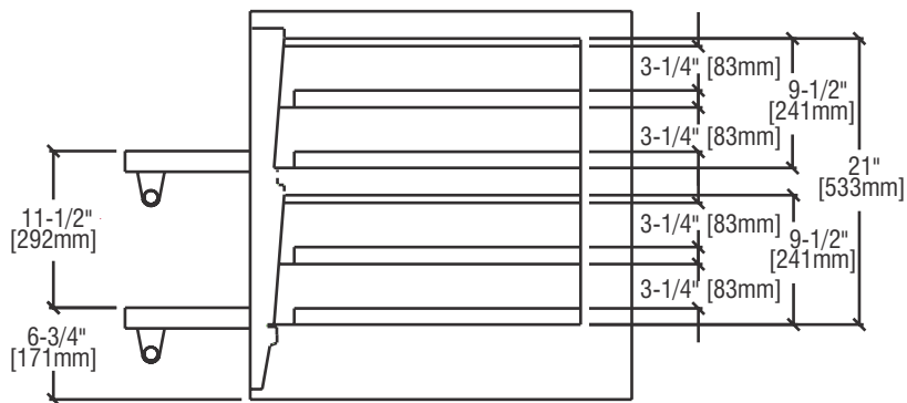
RH SIDE VIEW P44S
