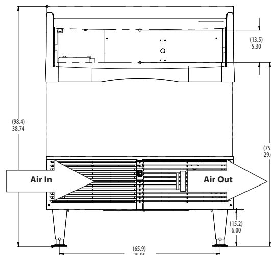
CU3030 front view
