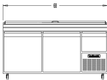
CPA68 FRONT VIEW
