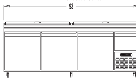
CPA93 FRONT VIEW
