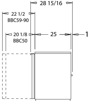
BBUC50,59,69,79 & 90 SIDE VIEW
