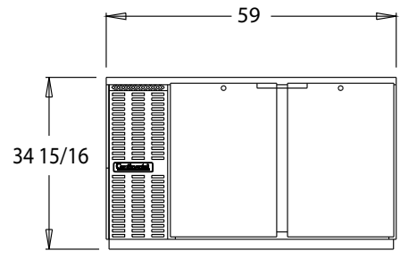
BBUC59 FRONT VIEW
