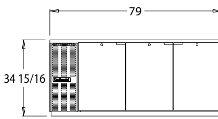
BBUC79 FRONT VIEW
