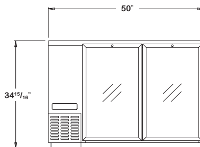
BBUC50-GD FRONT VIEW
