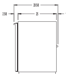
BBCU50,59,69,79 & 90 SIDE VIEW
