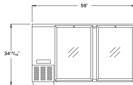
BBUC59-GD FRONT VIEW
