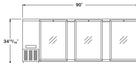
BBUC90-GD FRONT VIEW
